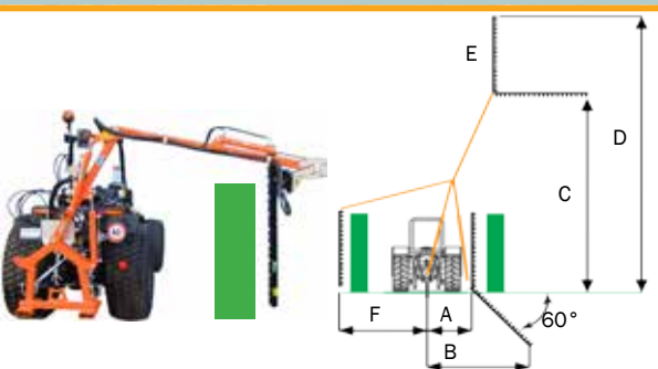
Snodo di sicurezza Safety brake away support Support de sécurité Sicherheitsgelenk Pojistný kloub
